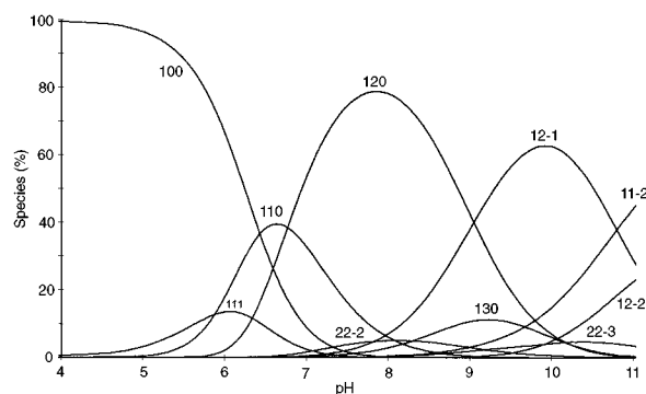
Fig. 6 Species distribution curves for the zinc(II)-aegaln 1:3 system calculated on the basis of the zinc(II) contents of the individual species ( [Zn^{2+}] = 0.01 \text{ mol dm}^{-3} )
