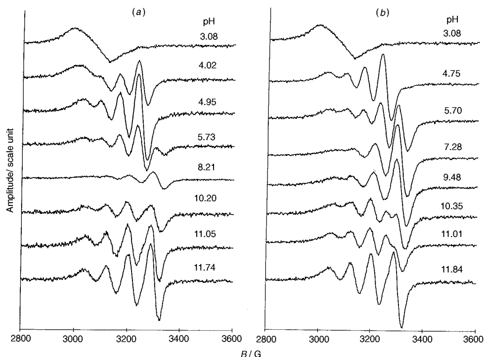
Fig. 2 The EPR curves for copper(II)-aegaln 1:1.25 (a) and 1:2.5 systems (b) ( [\text{Cu}^{2+}] = 0.005 \text{ mol dm}^{-3} ) systems as a function of pH
