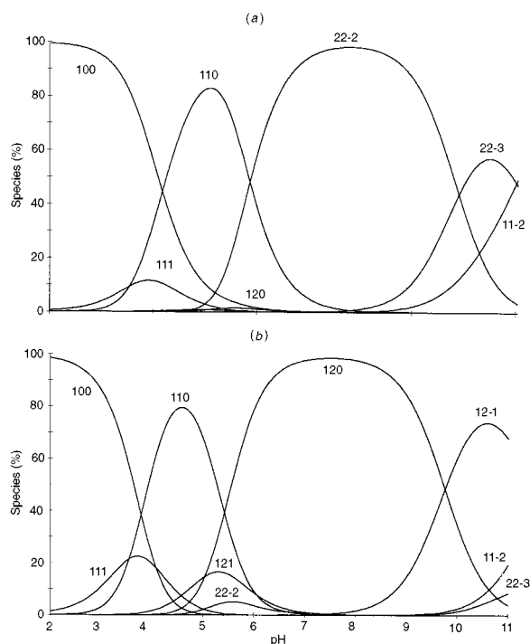
Fig. 1 Species distribution curves for the copper(II)-aegaln 1:1 (a) and 1:3 (b) systems calculated on the basis of the copper(II) contents of the individual species ( [\text{Cu}^{2+}] = 0.01 \text{ mol dm}^{-3} )
