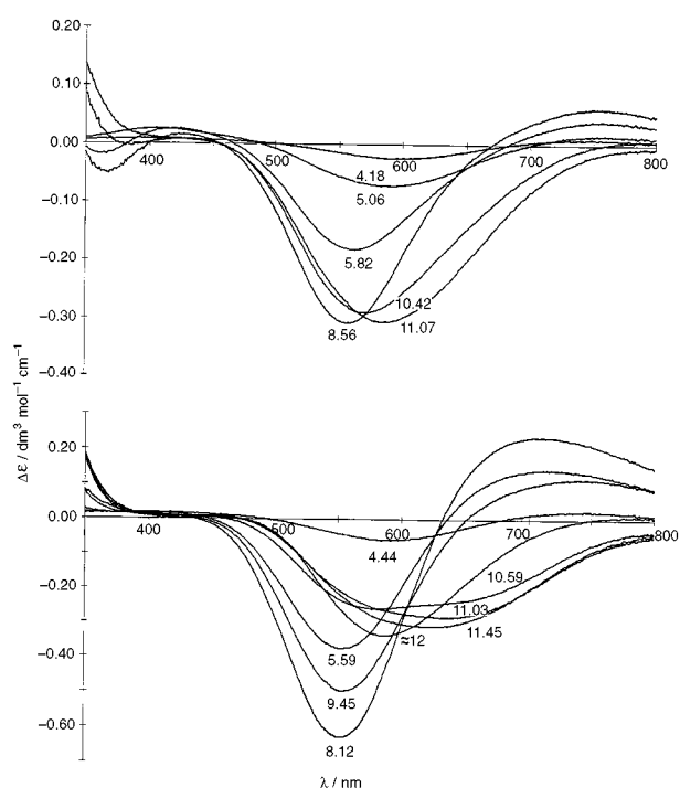
Fig. 3 Circular dichroism curves detected in copper(II)-aegaln 1:1 (a) and 1:2 (b) systems as a function of pH: ( [\text{Cu}^{2+}] = 0.005 \text{ mol dm}^{-3} )
